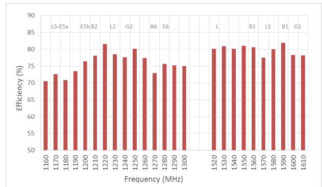
Figure 5 – Efficiency of the VP6000
